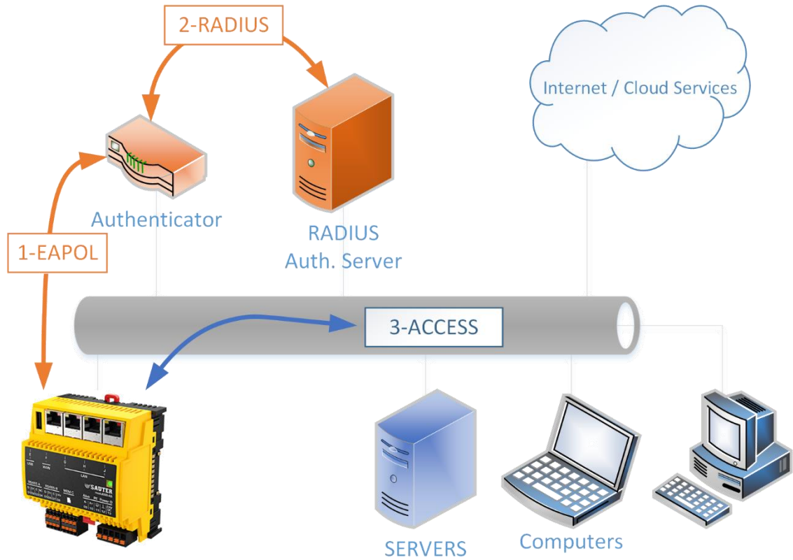
Figure 7 802.1X topology and protocols 1. Authorization Request 2. Identity check 3. Access to ressources
